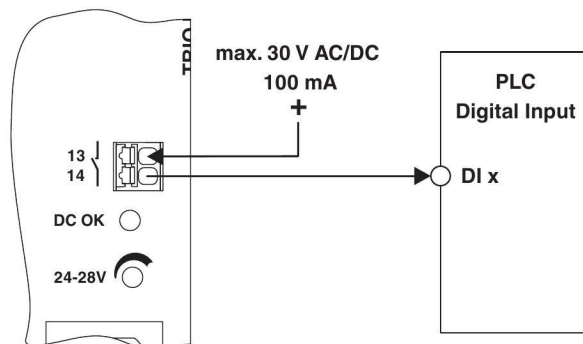
Figure 18 Wiring principle
