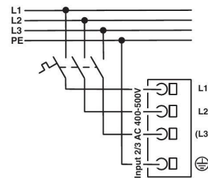
Figure 12 Schematic diagram, switching the input terminals
